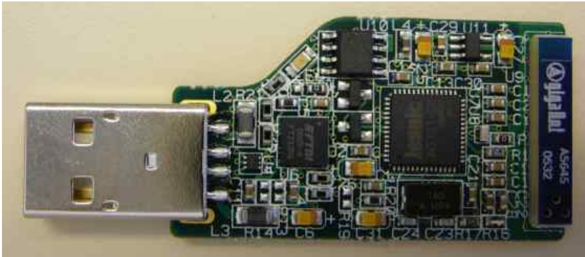
un-packaged USB dongle for ZigBee Wireless
